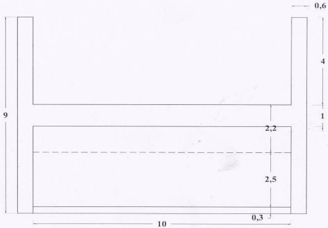
Construction of R.C.C. CD - 2 near to Coca Cola at Urawade
